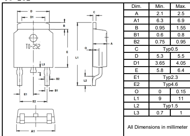
TO-252
