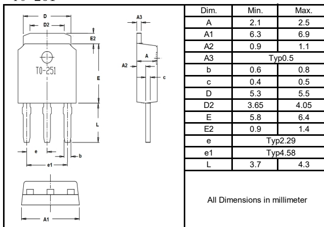
TO-251
